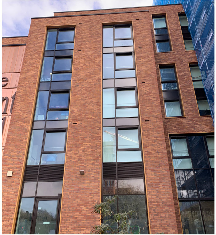
Figure 21: Brick slip façade
